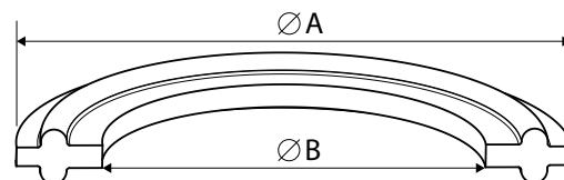
Unflanged type gasket for sizes >math>3/4''</math> flange OD
