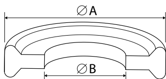
Unflanged type gasket for sizes <math>< 3/4''</math> flange OD
